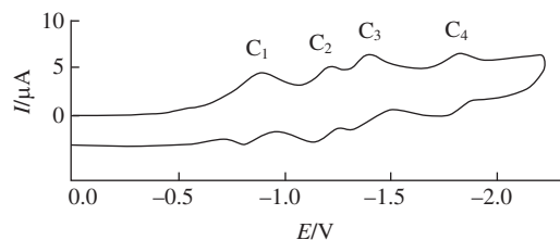
Figure 1 CV curve of methanofullerene 5 [recorded from 0.00 V to –2.30 V and back to 0.00 V; solution concentration 1 \times 10^{-3} mol dm^{-3} in o -DCB:MeCN (3:1); supporting electrolyte, 0.1 M Bu_4NBF_4 ; cathode, glassy carbon (GC) ( S_{\text{work}} = 3.14 mm 2 ); reference electrode, Ag/AgNO 3 0.01 M in MeCN; scan rate, V_{\text{pot}} = 50 mV s^{-1} ].
